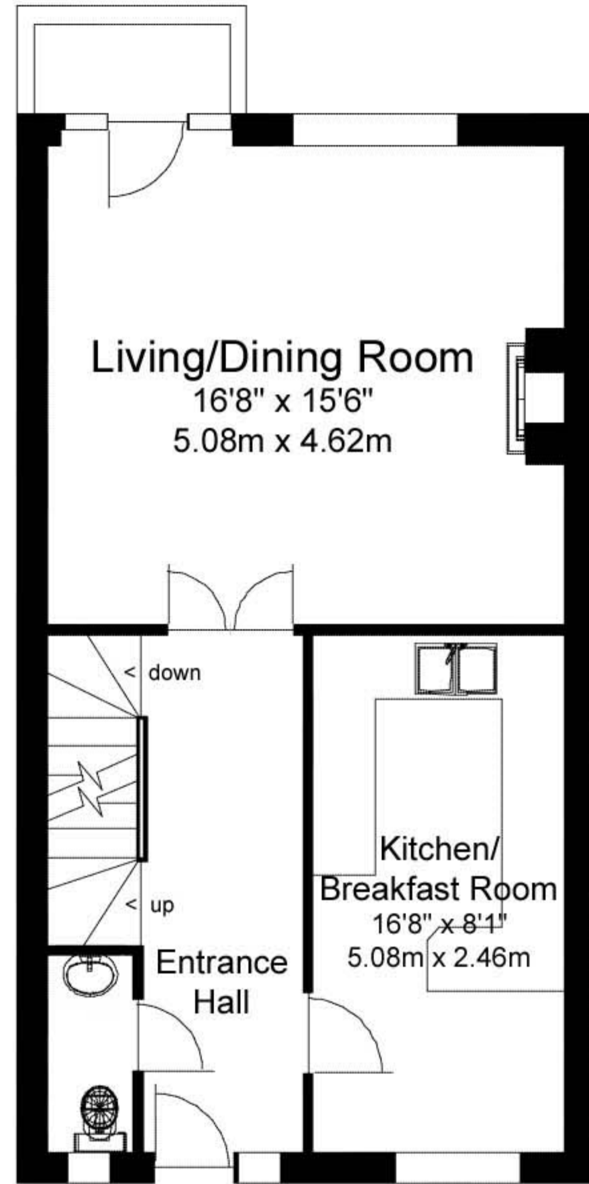
UPPER GROUND FLOOR
